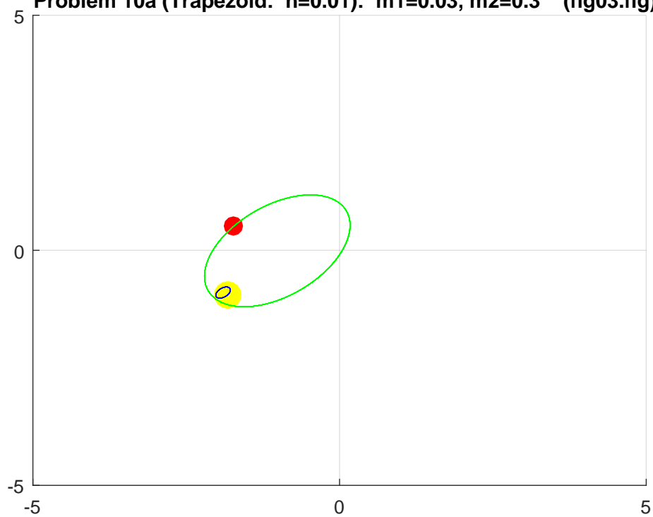
Celestial Mechanics: Two (2) Body Problem Problem 10a (Trapezoid: h=0.01 ): m_1=0.03 , m_2=0.3 (fig03.fig)
